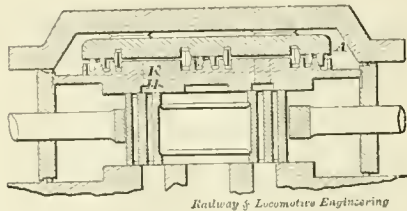
Fig. 4.—EXHAUST JUST OPENING AT LEFT.
